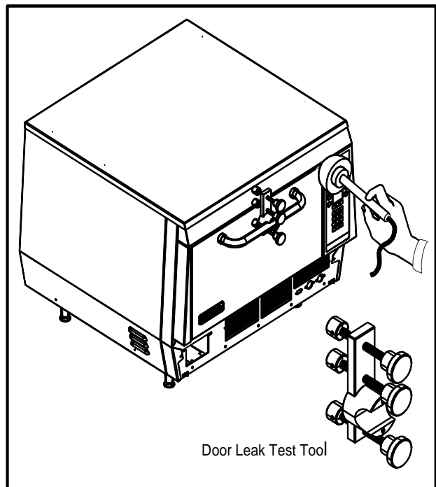
FIGURE 9 - 1 Microwave Leakage Testing
